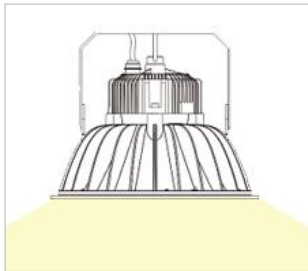
120° stralingshoek
